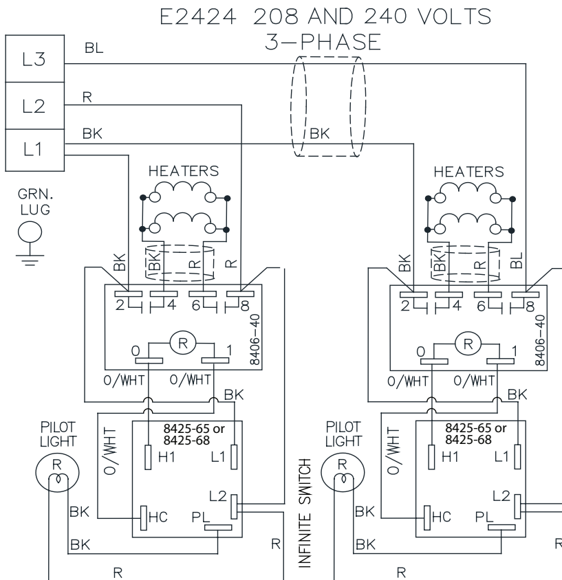
Figure 2A - E2424 Schematics for 208 V and 240 V Single-Phase and 3-Phase
