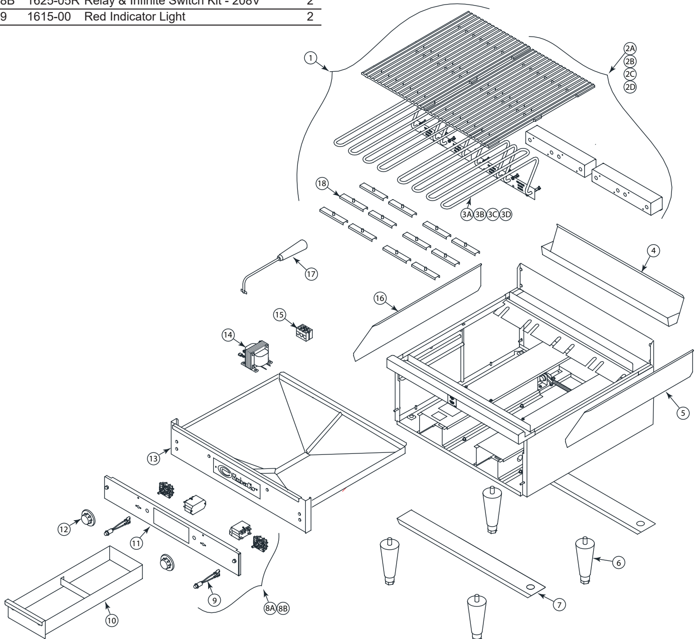
Figure 3 - E2424 Exploded View
