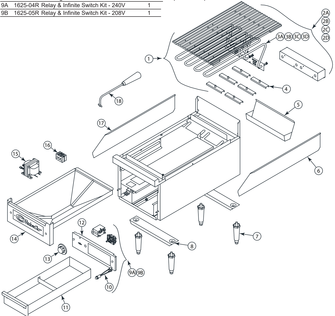
Figure 3 - E2412 Exploded View
