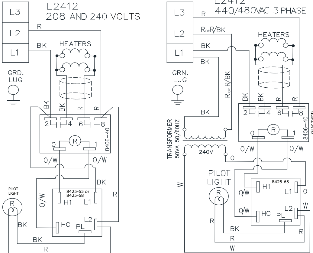
Figure 2 - E2412 Schematics for - 208V, 240V, 440V and 480V
